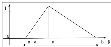
Fig 2: Triangular Fuzzy Membership Number
