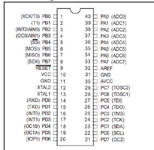
Figure 5: ATMEGA16
