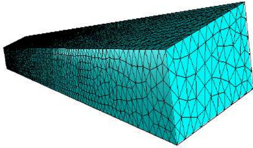
Figure 6: Triangular meshes in Elmer
