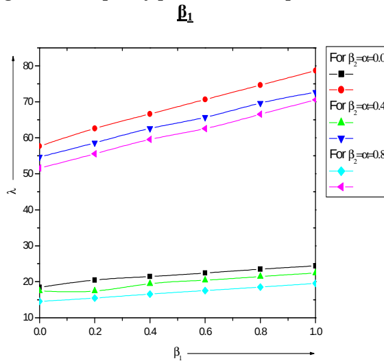
Figure 3:- Frequency parameter vs taper constant
