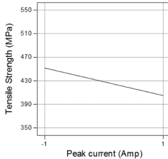
Fig.4.1 Effect of Peak current on Tensile Strength
