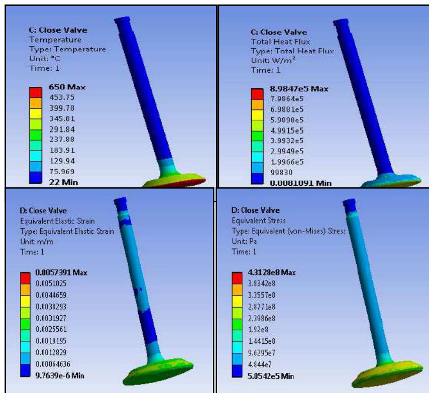
Figure 11 Results plots for closed engine valve coated with 200 \mu\text{m} \text{CaZrO}_3
