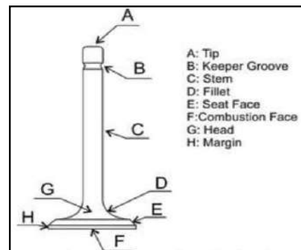
Figure 1 Descriptive image of Engine valve
