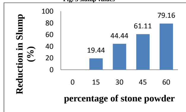
Fig. 4 percentage decrease in slump
