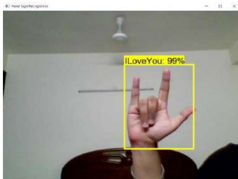
Fig.2andFig.3aresomeoutputsfromtheHand SignRecognitionSystem
